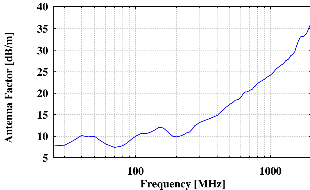
Antenna Factor
