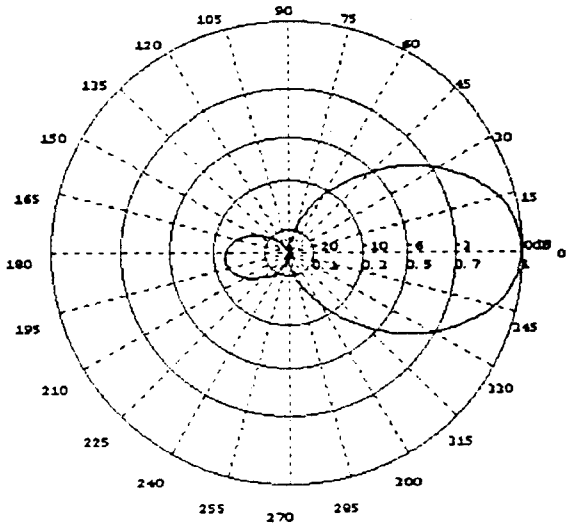
E-Ebene 135 MHz E Plane 135 MHz
