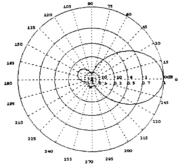
E-Ebene 180 MHz E Plane 180 MHz
