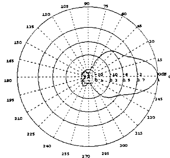
E-Ebene 1000 MHz E-Plane 1000 MHz
