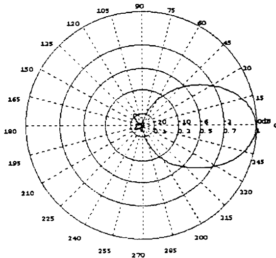
E-Ebene 700 MHz E-Plane 700 MHz
